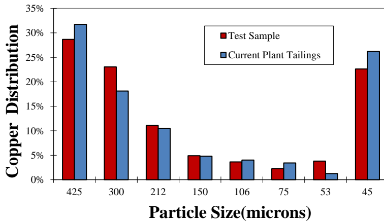
Figure 6. Copper distribution by size for plant and as-received samples
