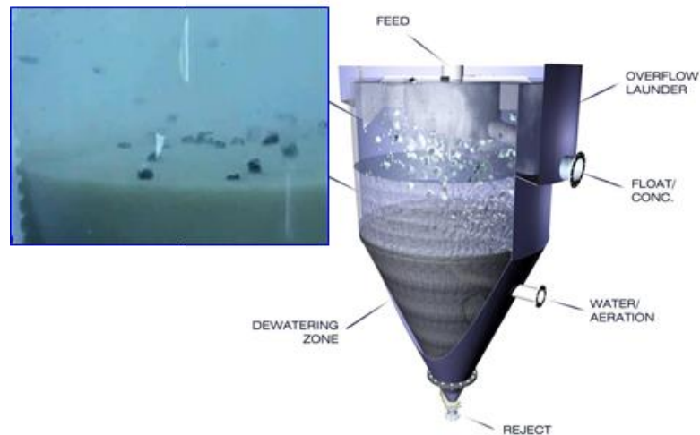
Figure 3 – Schematic illustration of HydroFloat™ separator
