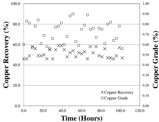
Figure 9 – Long-term pilot circuit test
