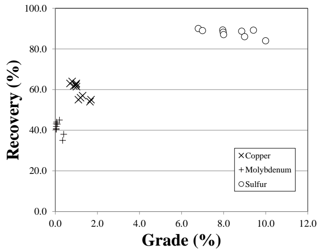
Figure 7. Laboratory results for coarse particle HydroFloat™ flotation test work
