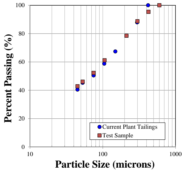
Figure 5. Particle size distribution for test sample and current production tailings
