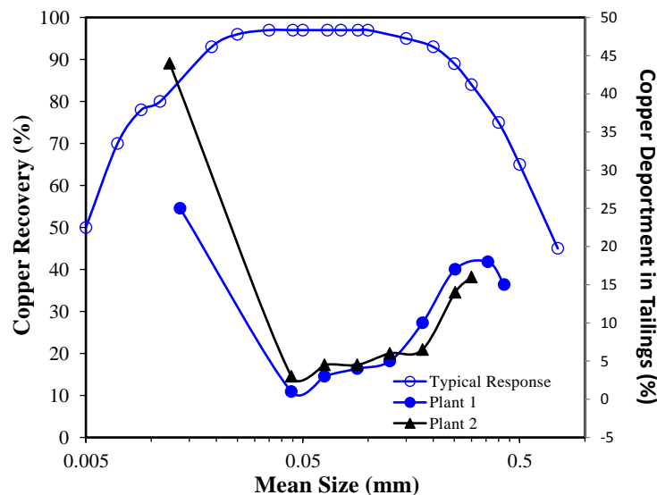
Figure 1 - Typical conventional flotation response and corresponding deportment of pay metals in tailings
