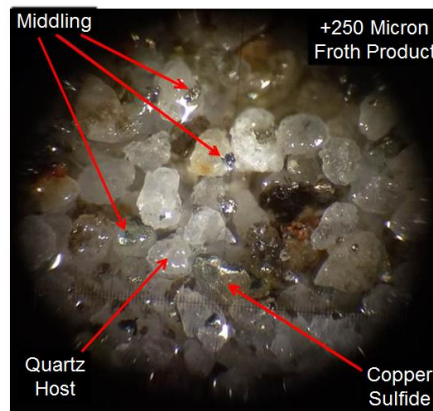
Figure 2 – Photo of middling particles recovered from tailings using the HydroFloat™ technology
