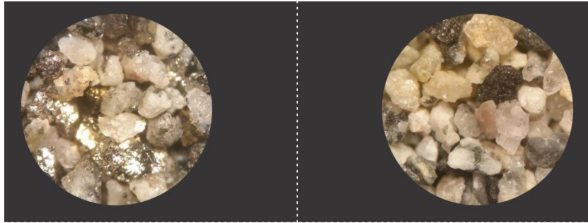
Figure 8 - Microscopic view of +425 concentrate (left) and tailings (right) particles
