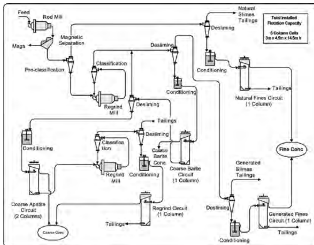
FIGURE 9 Phosphate flotation circuit using columns
