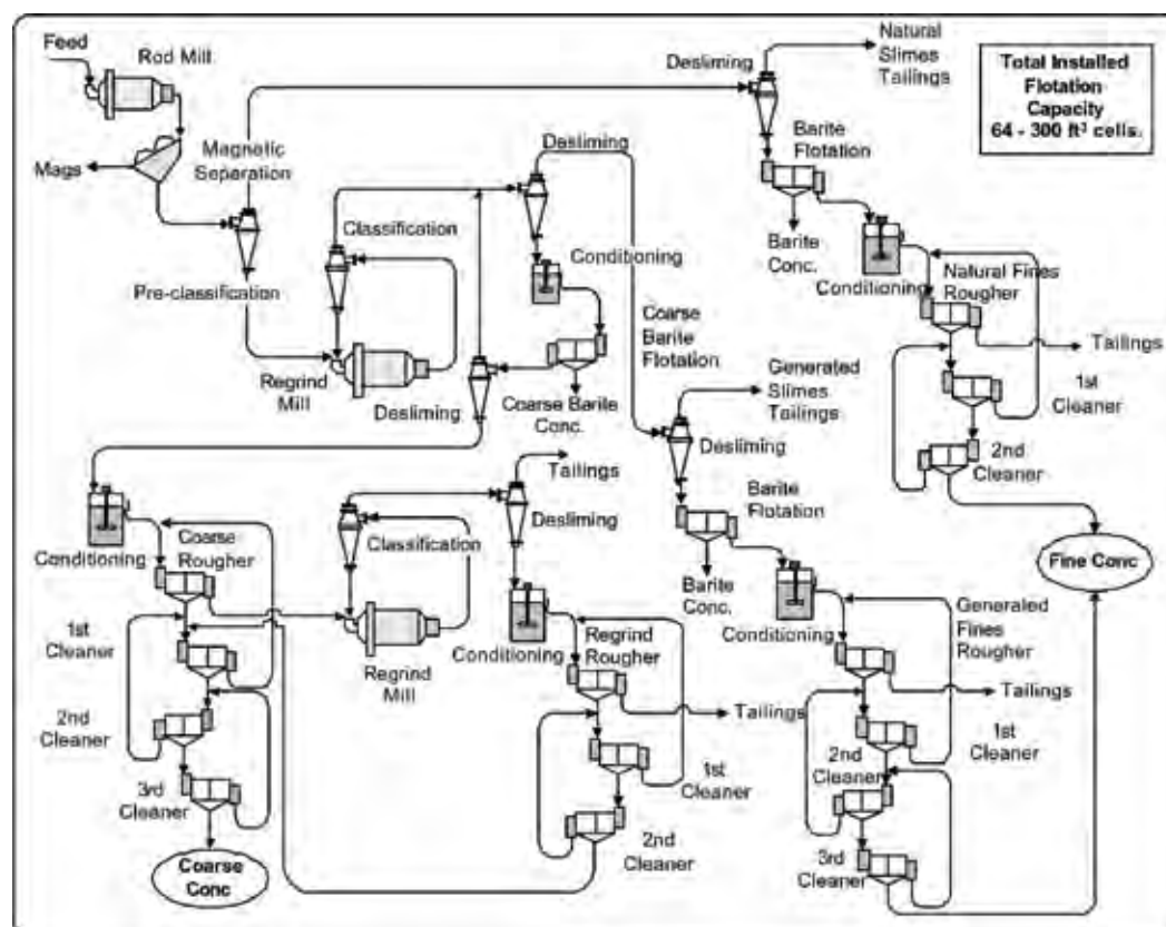
FIGURE 8 Phosphate flotation circuit using mechanical cells
