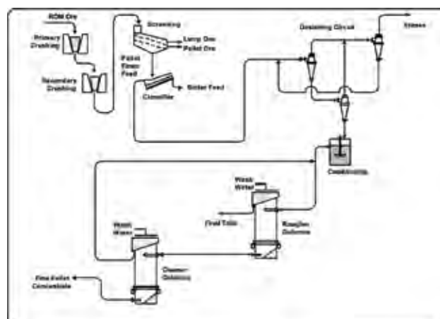
FIGURE 3 Flotation circuit using column cells
