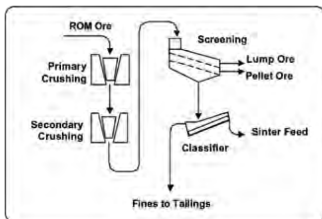
FIGURE 1 Typical iron ore processing flowsheet
