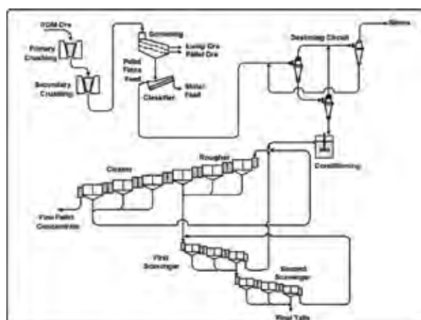
FIGURE 2 Flotation circuit using mechanical cells
