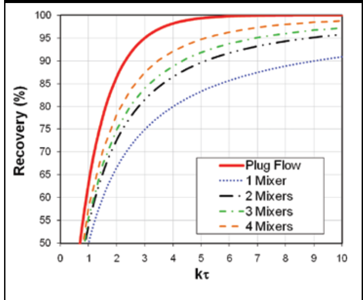
Figure 1 - Recovery Versus k\tau for Various Circuit Configurations.
