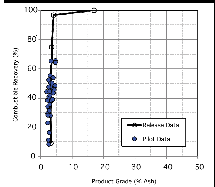
Figure 6 - Single-Stage Treatment of Red Ash, Gilbert and Pocahontas No. 3 Seams.
