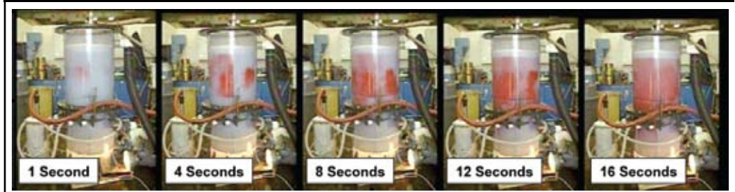
Figure 2 - Photographs Showing Axial Dispersion in a Column Cell.
