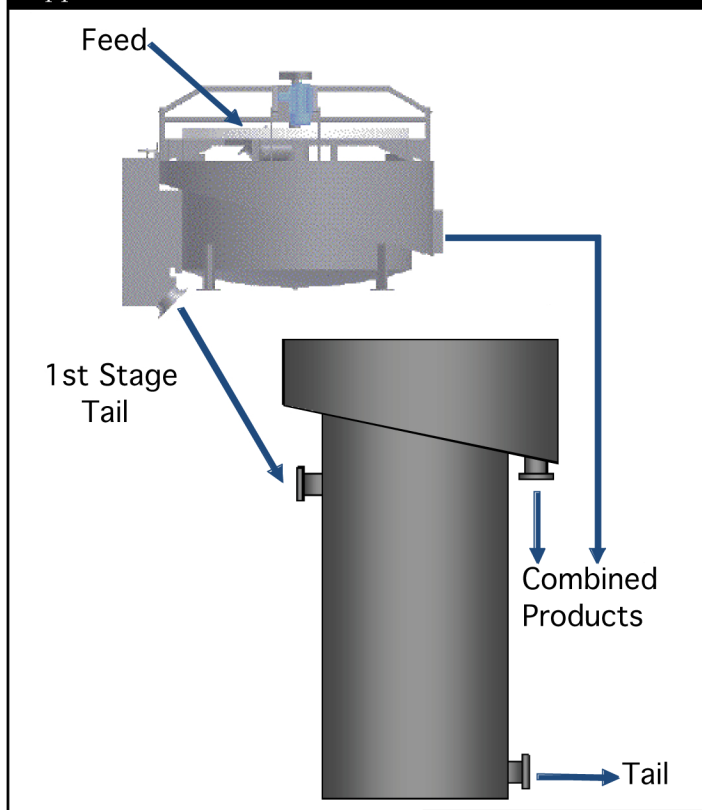
Figure 11 - New Cell Arrangement for Slow Floating Applications.
