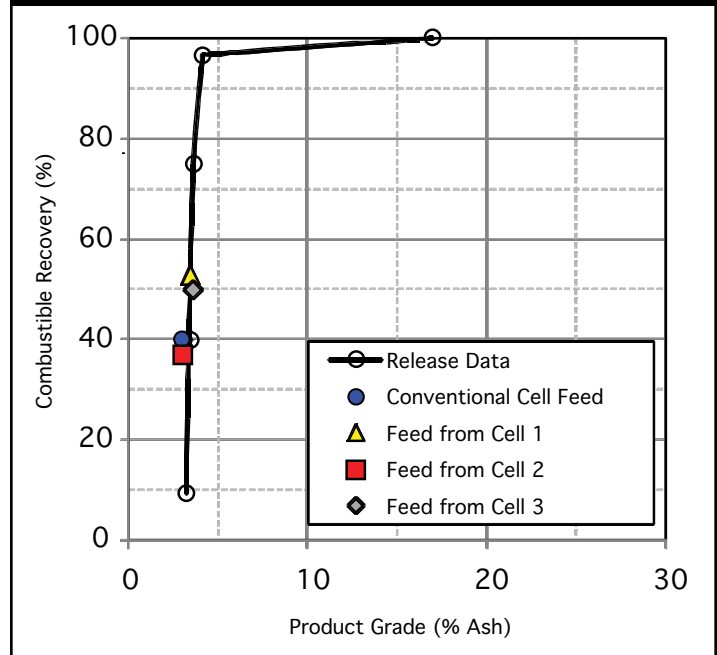
Figure 8 - Average Recovery for Various Feed Points of a Conventional Cell.
