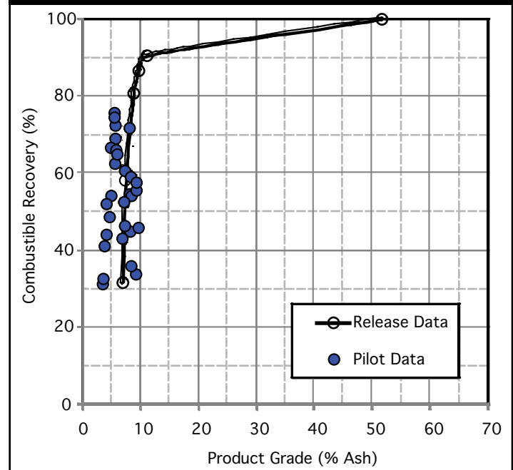
Figure 5 - Single-Stage Treatment Amburgy and Hazard No. 4 Seams.
