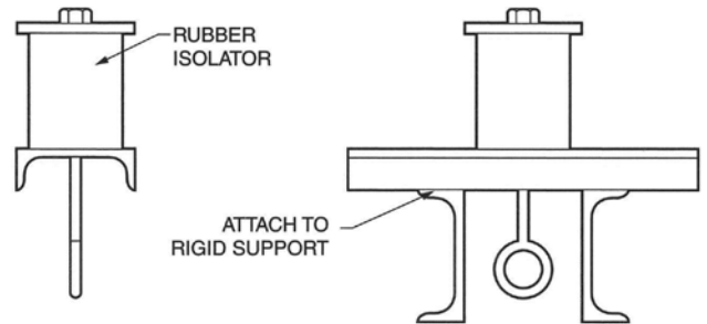
Figure 1 Typical Suspension Isolator
