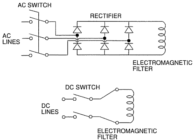
FIGURE 3. BASIC ELECTRICAL SCHEMATIC
