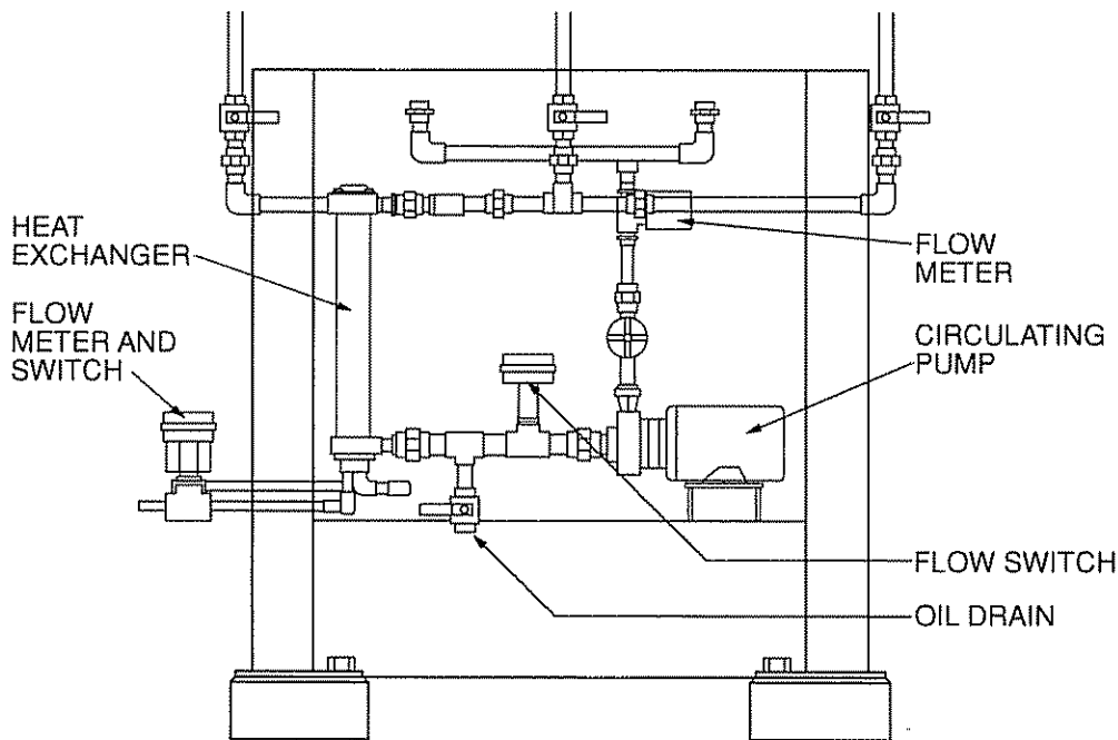
FIGURE 5. TYPICAL FORCED COOLING SYSTEM
