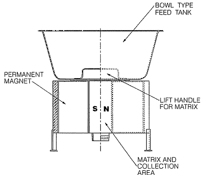
FIGURE 4. PERMANENT MAGNET BOWL TYPE HI FILTER
