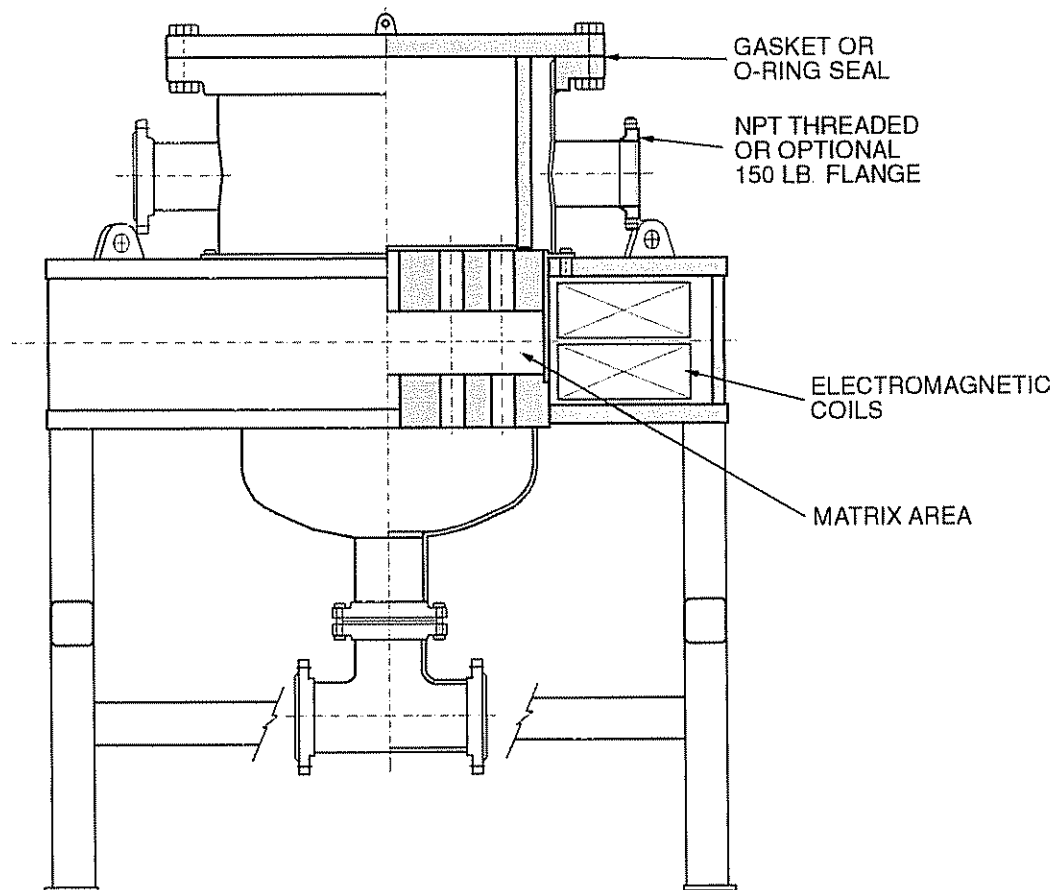
FIGURE 1. TYPICAL 2,500 GAUSS HI FILTER
