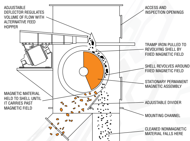
Figure 1. Permanent Magnetic Drum Separators
