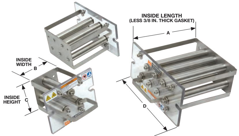
RARE EARTH DRAWER MAGNETS (INCHES)
